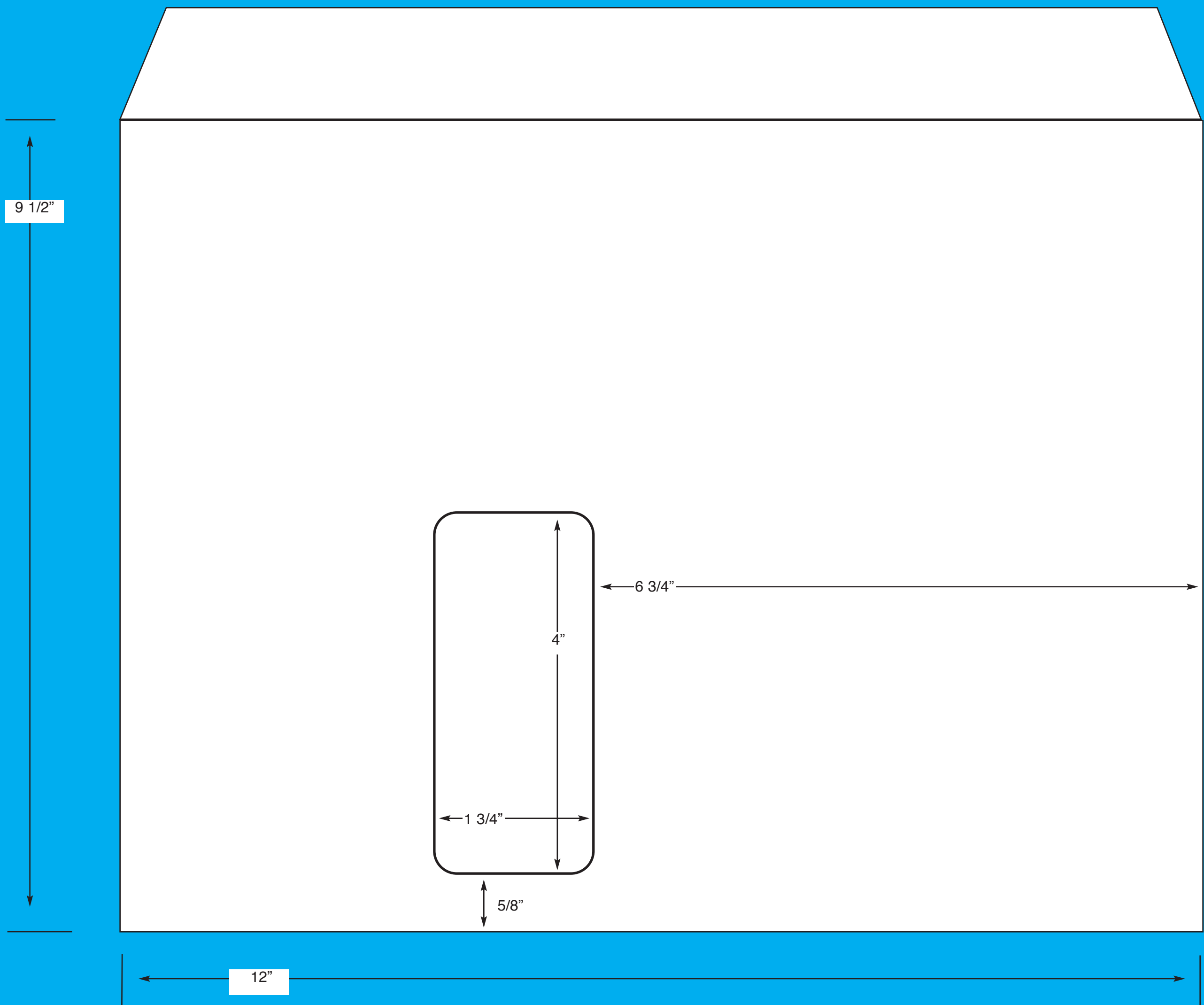
SF-13 9 1/2" x 12" window
